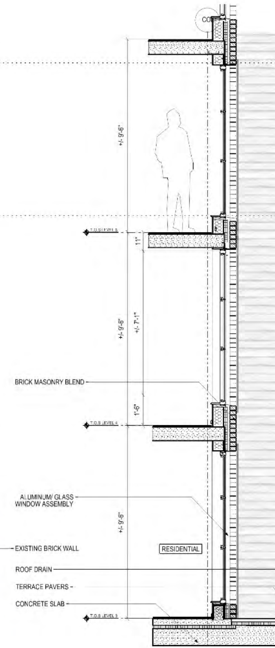
SECTION
