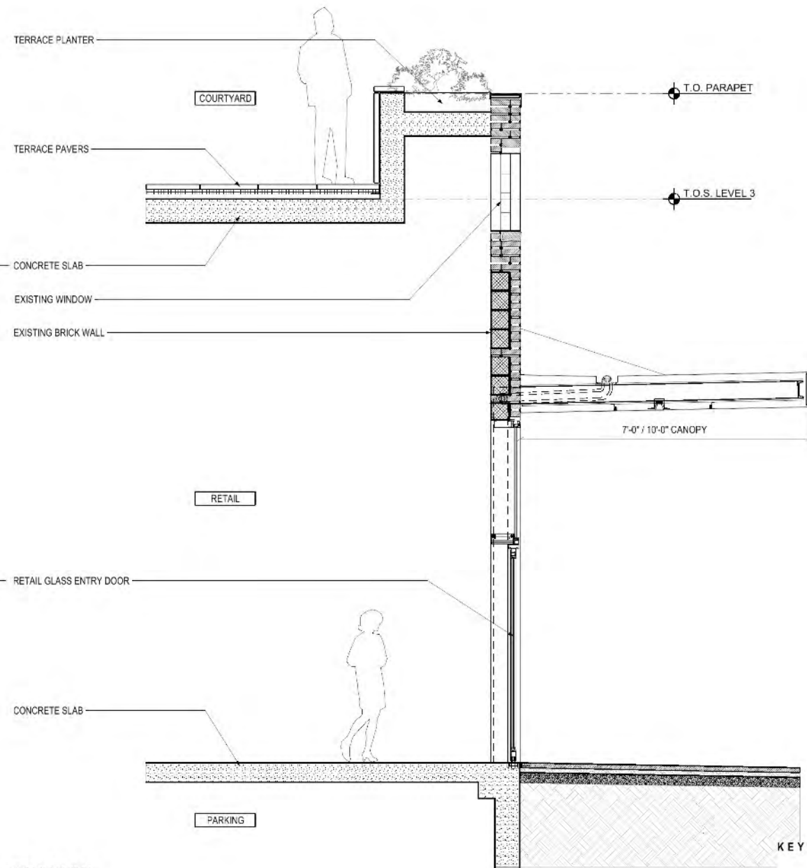
SECTION
