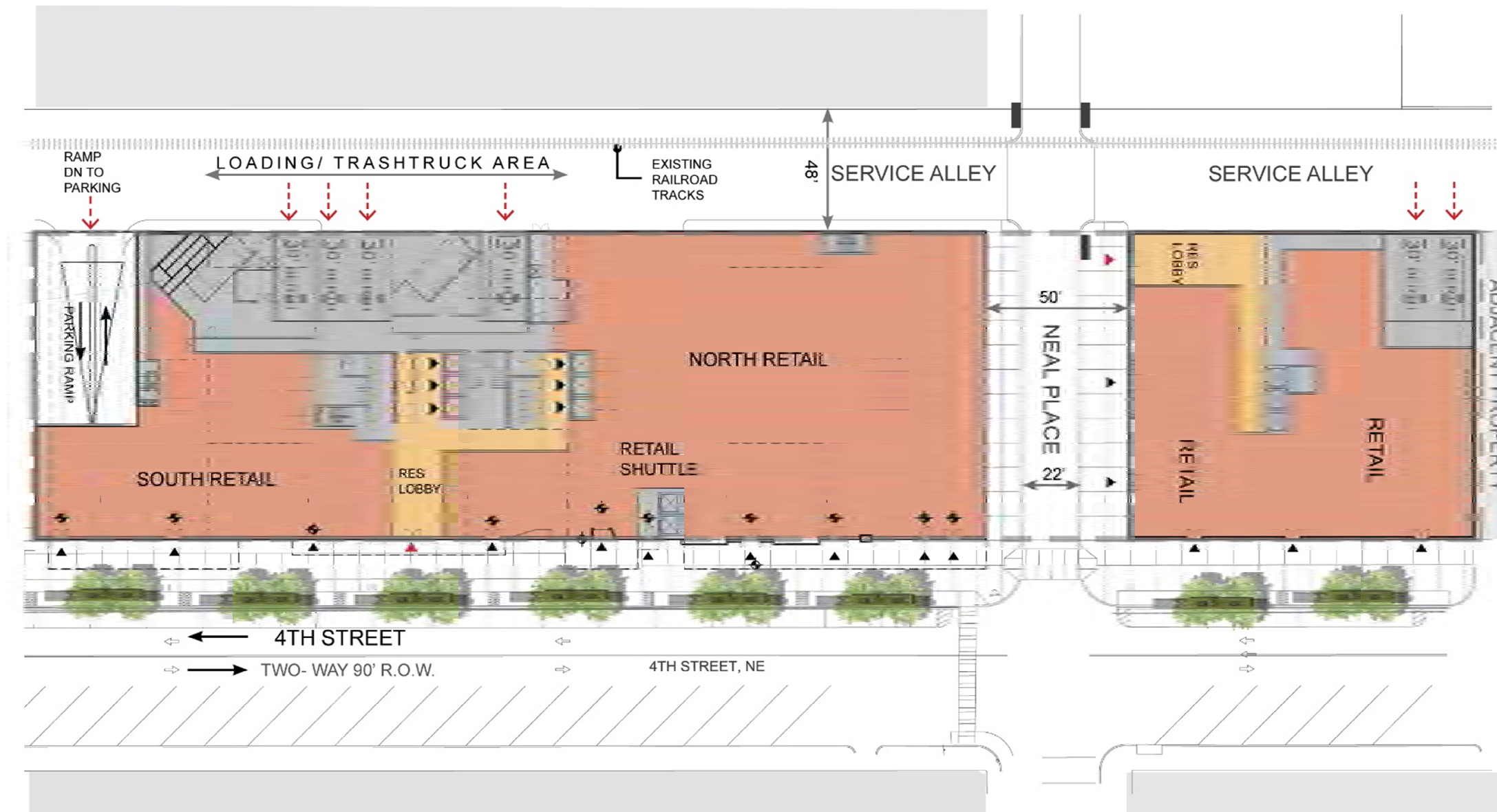
GROUND PLAN
